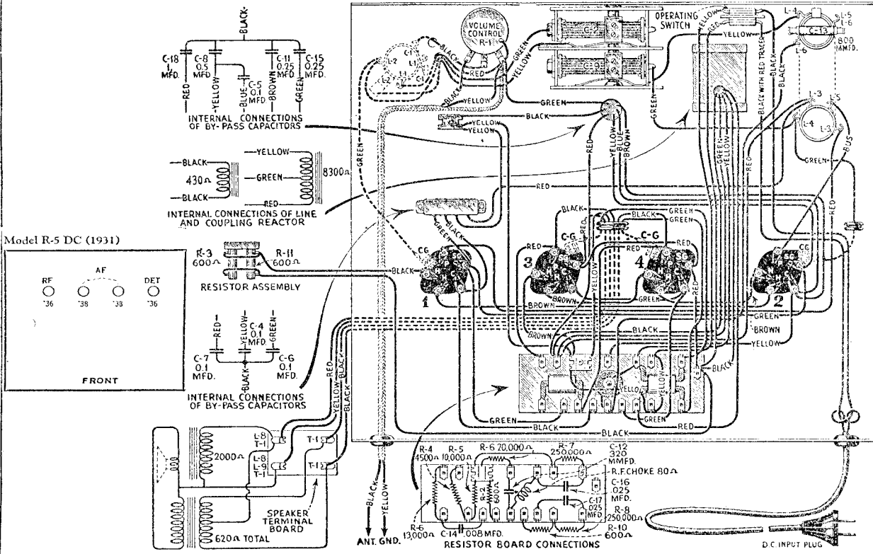
Figure 2—Wiring Diagram
